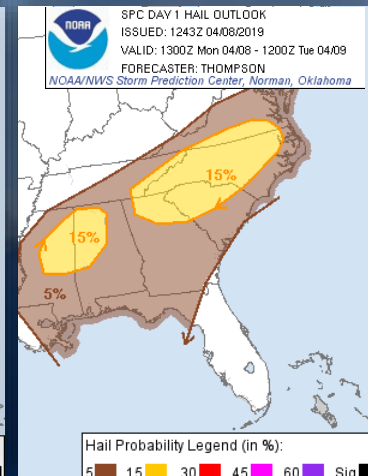
Hail Probability
